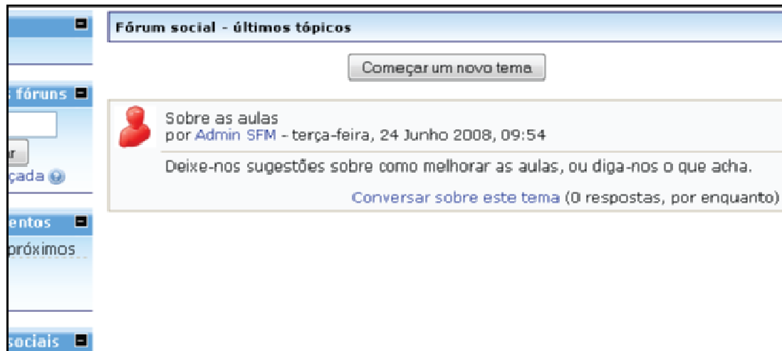
Figura 11 -Disciplina Social
